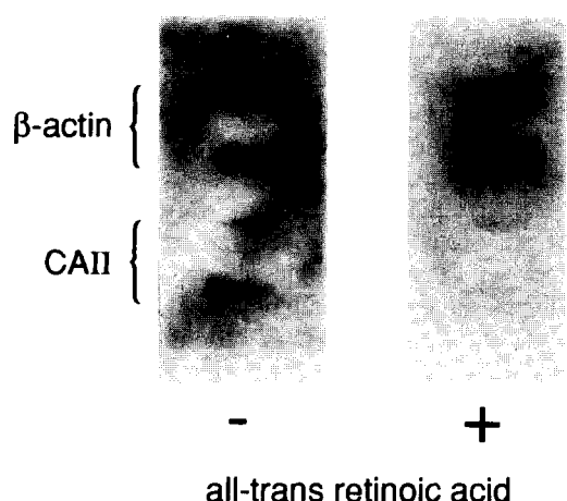
Fig. 5. Effects of ATRA on CA II gene transcription in DANG cells. DANG cells were incubated with 10 \mu M ATRA or vehicle for 48 h and CA II and \beta -actin transcription were assessed by nuclear run on assays. Duplicate slots for each cDNA were hybridised to ensure the reproducibility. Shown is a representative of 3 independent experiments yielding nearly identical results.
